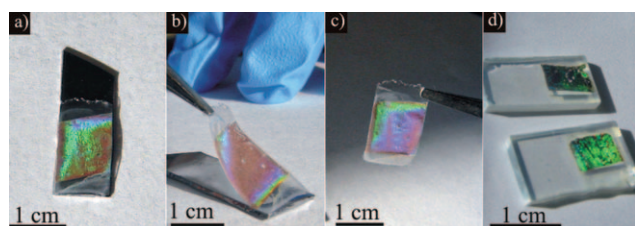
Figure 2. Photographs of stages of the transfer process of a silicon photonic crystal. a) The silicon photonic film on its original substrate after underetching with HF. b) The film is gently peeled from the substrate with tweezers. c) The preformed film is ready to be deposited onto any substrate. d) Inverse Si opals on dye sensitized ZnO NW electrodes after calcination at 500 °C for 2 h.
